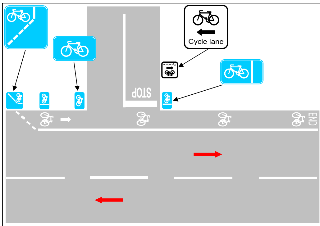
Figure 12 : Typical Signage Layout for Cycle Routes
