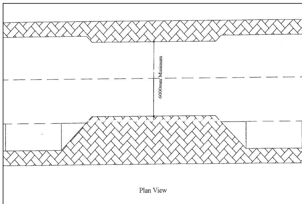
Figure 21 : Build Outs
