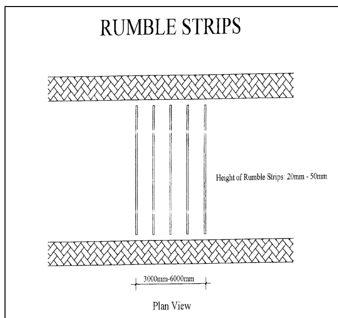
Figure 14 : Rumble Strips
