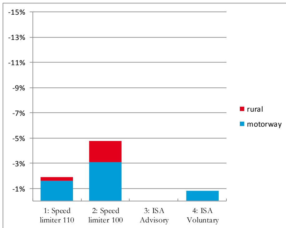
Figure 6-4: CO 2 emission effects for different emissions – LCV scenarios
