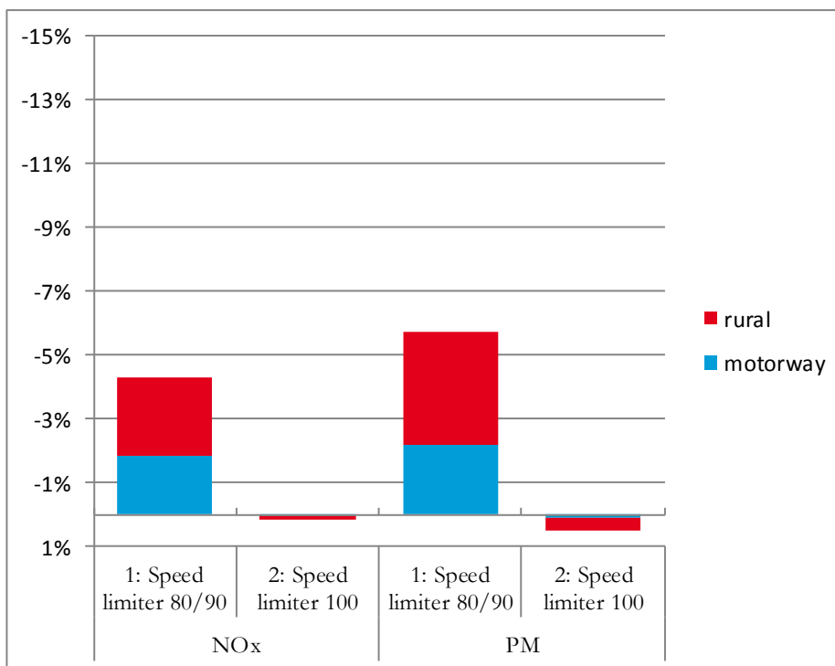
Figure 5-5: Emission effects for NO x and PM emissions – HCV scenarios 1 and 2
