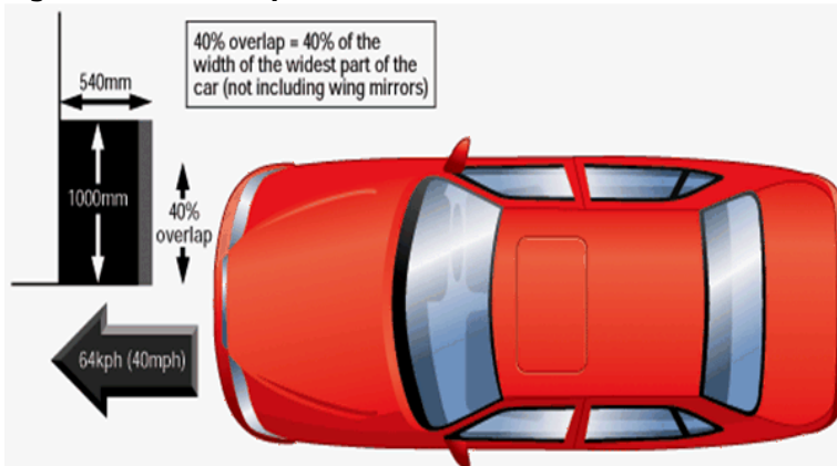
Figure 4: Frontal impact test
